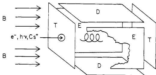
Figure 1. Schematic diagram of the sample chamber ("cell") in an ion cyclotron mass spectrometer. See text for distinctions between omegatron, ICR, and FT/ICR.
